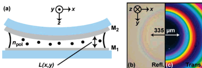
Figure 1. Optical microresonator doped with single-walled carbon nanotubes (SWNTs). (a) The sample consists of two mirrors, M_{1,2} , prepared by evaporating silver films onto glass coverslips. The mirrors are separated by a layer of a transparent polymer (PMMA) with varying thickness enclosing homogeneously distributed and randomly oriented SWNTs that are indicated by dots. Optical micrographs show the microresonator center illuminated with white light in (b) reflection and (c) transmission on M_1 . The local mirror spacing L(x,y) is extracted from (c) using eq 1 and served to calculate the normalized Raman scattering cross sections \sigma_{\text{cav}}(L)/\sigma_0 of embedded SWNTs shown in Figure 4.
